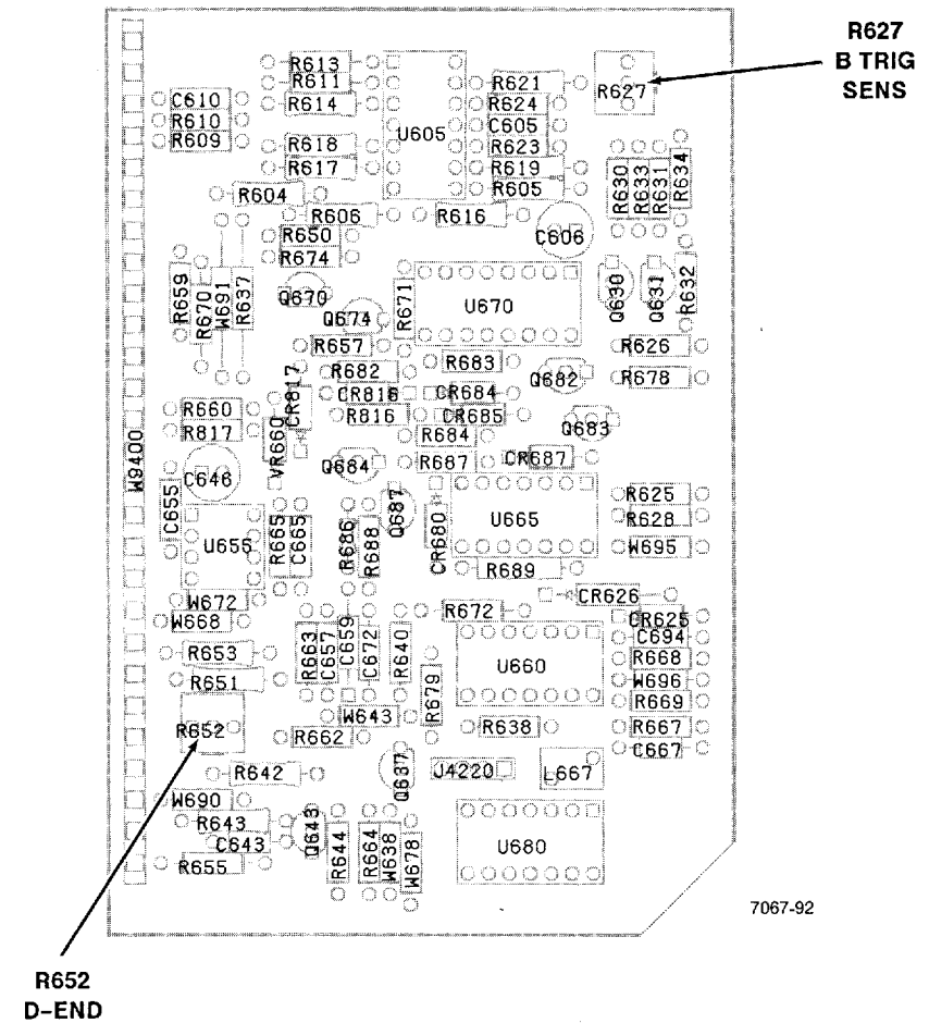
Figure 9-29. A5—Alt Sweep Logic board adjustment locations.
