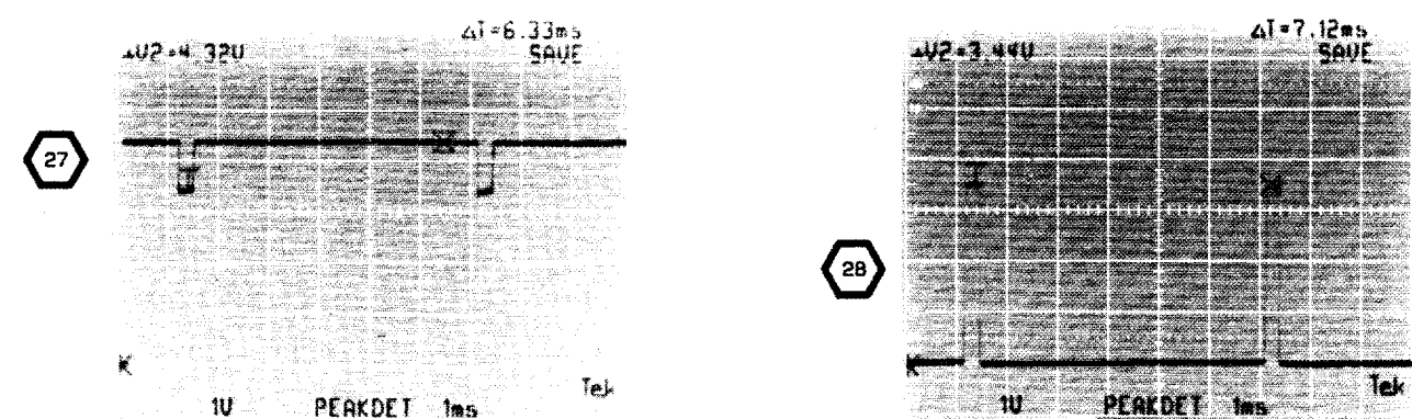
TEST SCOPE TRIGGERED ON U506 PIN 3 FOR WAVEFORMS 27 THROUGH 30
