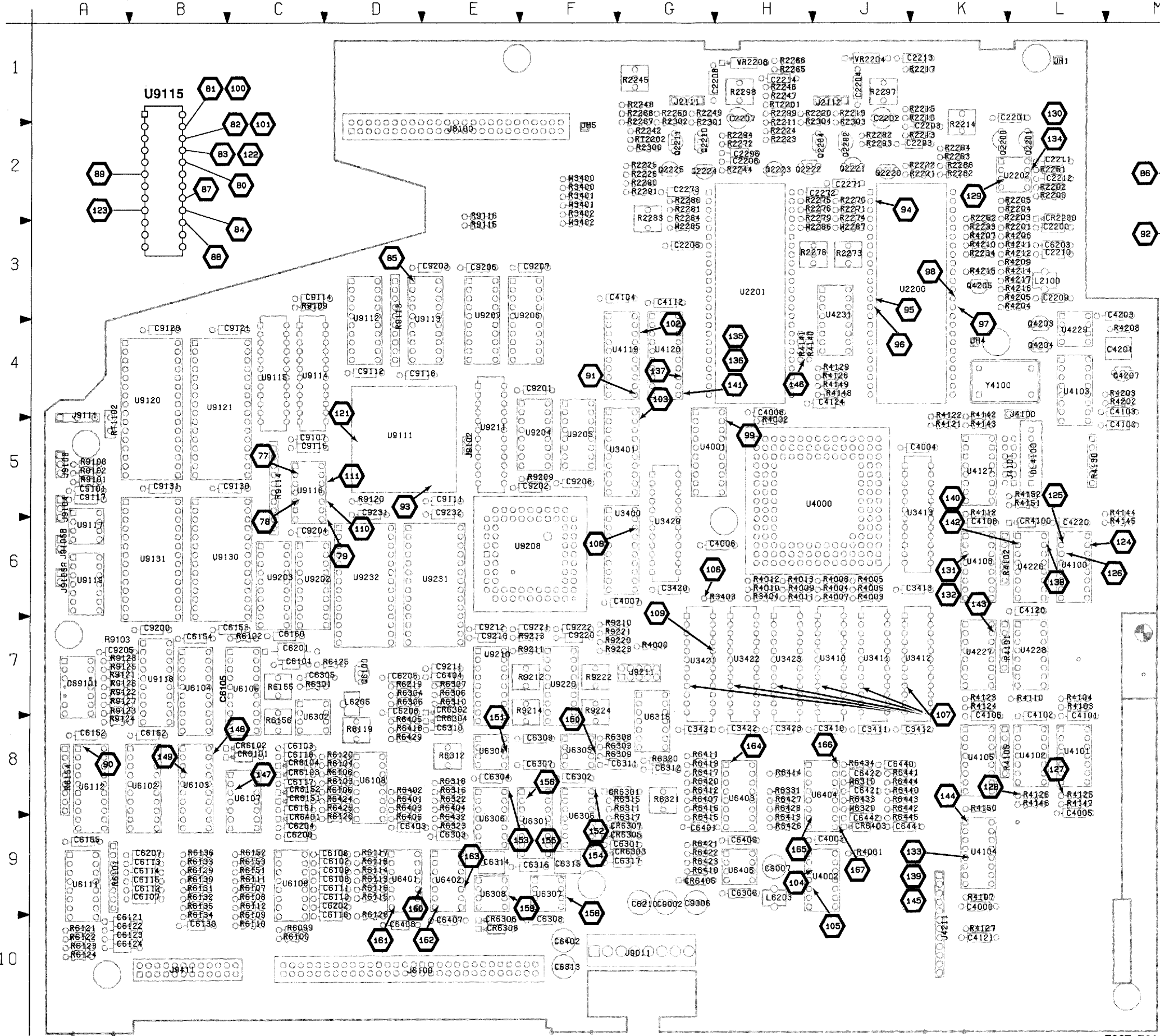
Figure 9-22. A10—Storage board.
