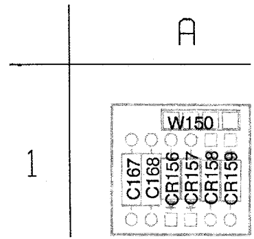
Figure 9-12. A1A9—CH 2 Bandwidth Limit board.
