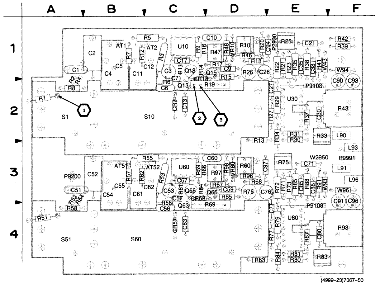
Figure 9-6. A2—Attenuator board.
