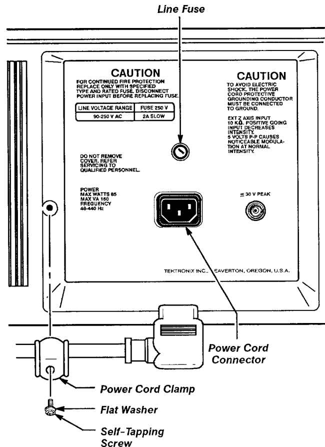
Figure 2-1. Securing the detachable power cord to the instrument.
