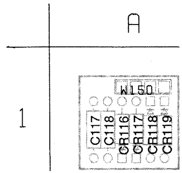
Figure 9-11. A1A8—CH 1 Bandwidth Limit board.
