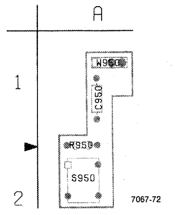
Figure 9-20. A1A18—Thermal Shutdown board. 7067-72
