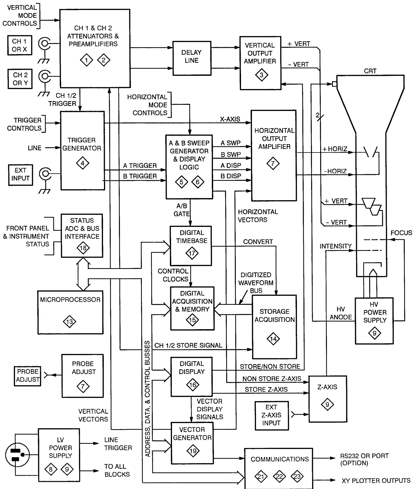
Figure 3-1. Simplified block diagram.
