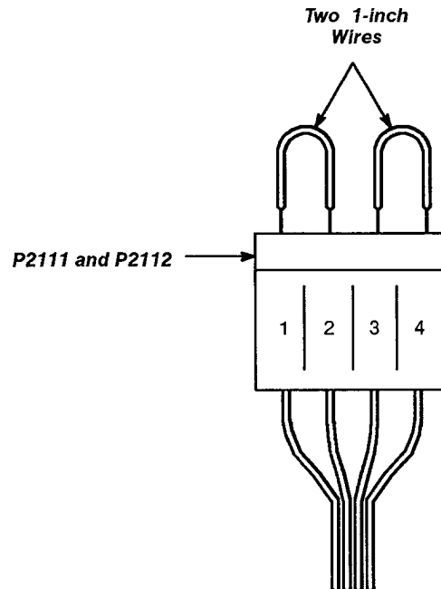
Figure 6-2. Grounding the signal lines of P2111 and P2112.
