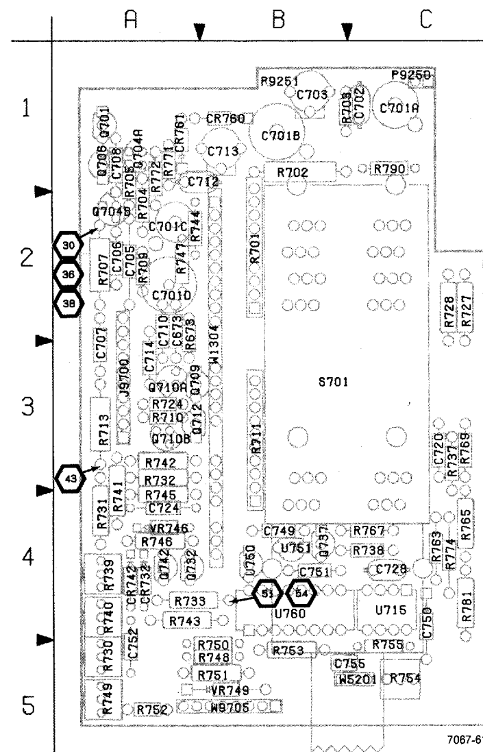
Figure 9-15. A4—Timing board.
