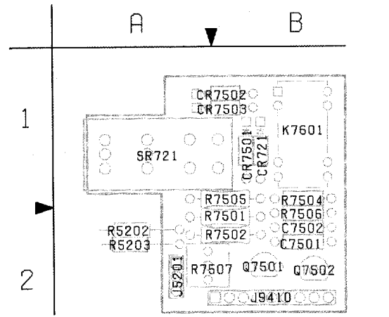
Figure 9-18. A16—Sweep Reference board.
