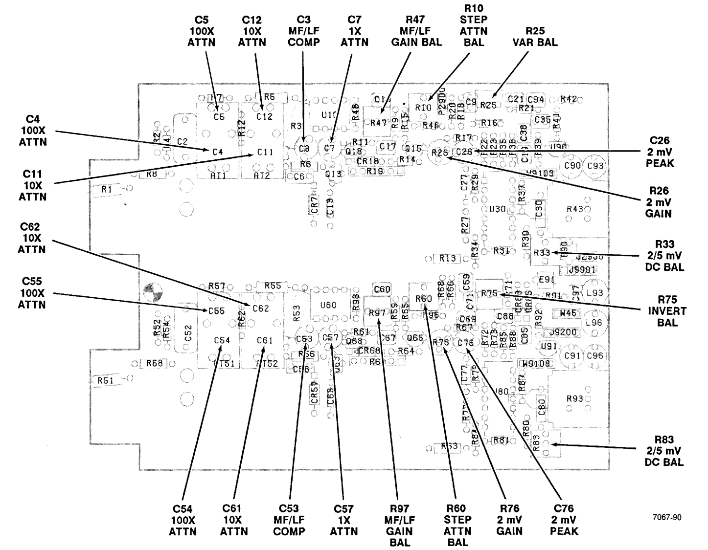
Figure 9-27. A2—Attenuator board adjustment locations.
