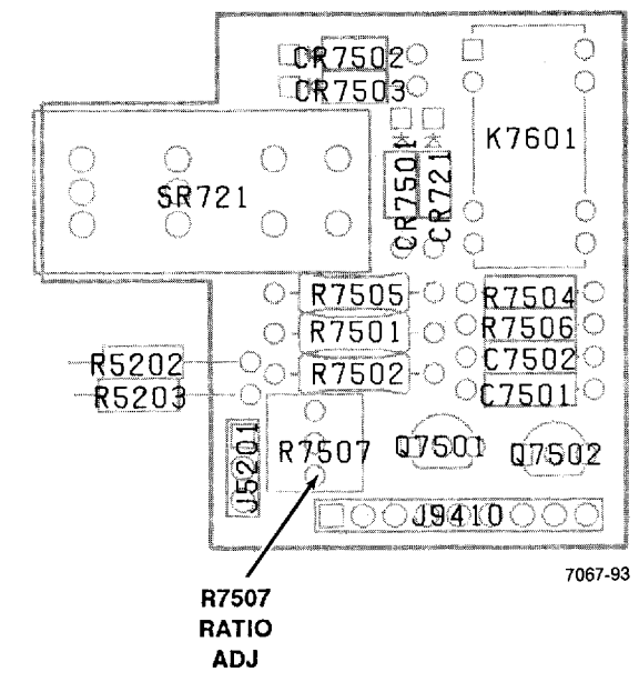
Figure 9-30. A16—Sweep Reference board adjustment locations.
