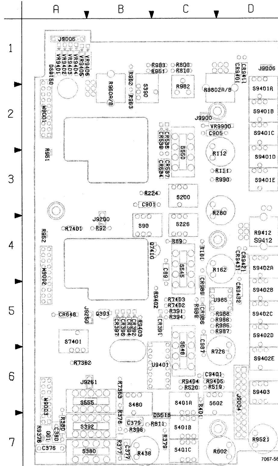
Figure 9-13. A3—Front Panel board.
